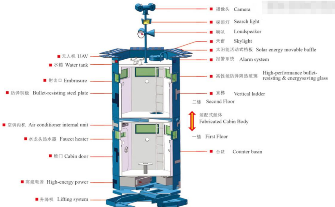
双层六边海岛型战防保安仓结构配置图 Structure of the Double-floor Hexagon Security Cabin for Warfare and Defense with Off Grid Self Power System
