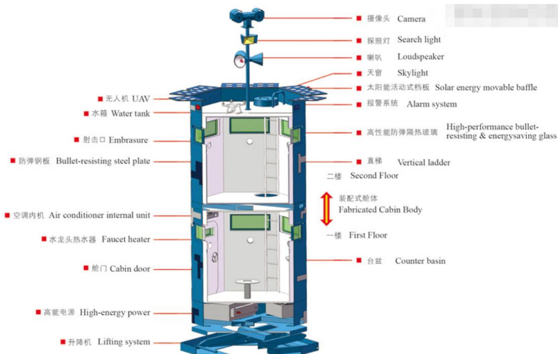
双层六边海岛型战防保安仓结构配置图 Structure of the Double-floor Hexagon Security Cabin for Warfare and Defense with Off Grid Self Power System
